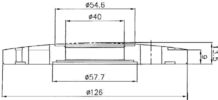
Valve Plate
