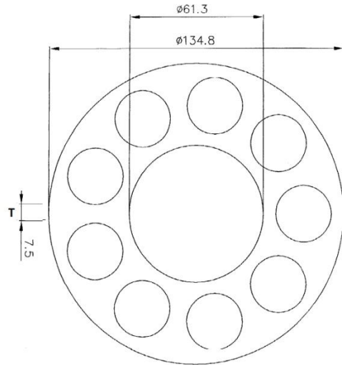
Set Plate
