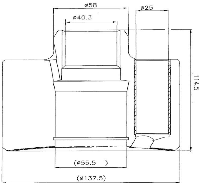
Cylinder Block
