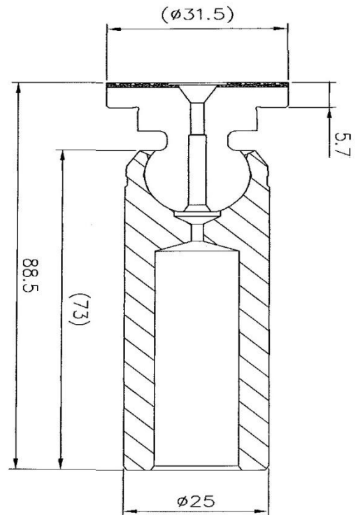
Piston Assy
